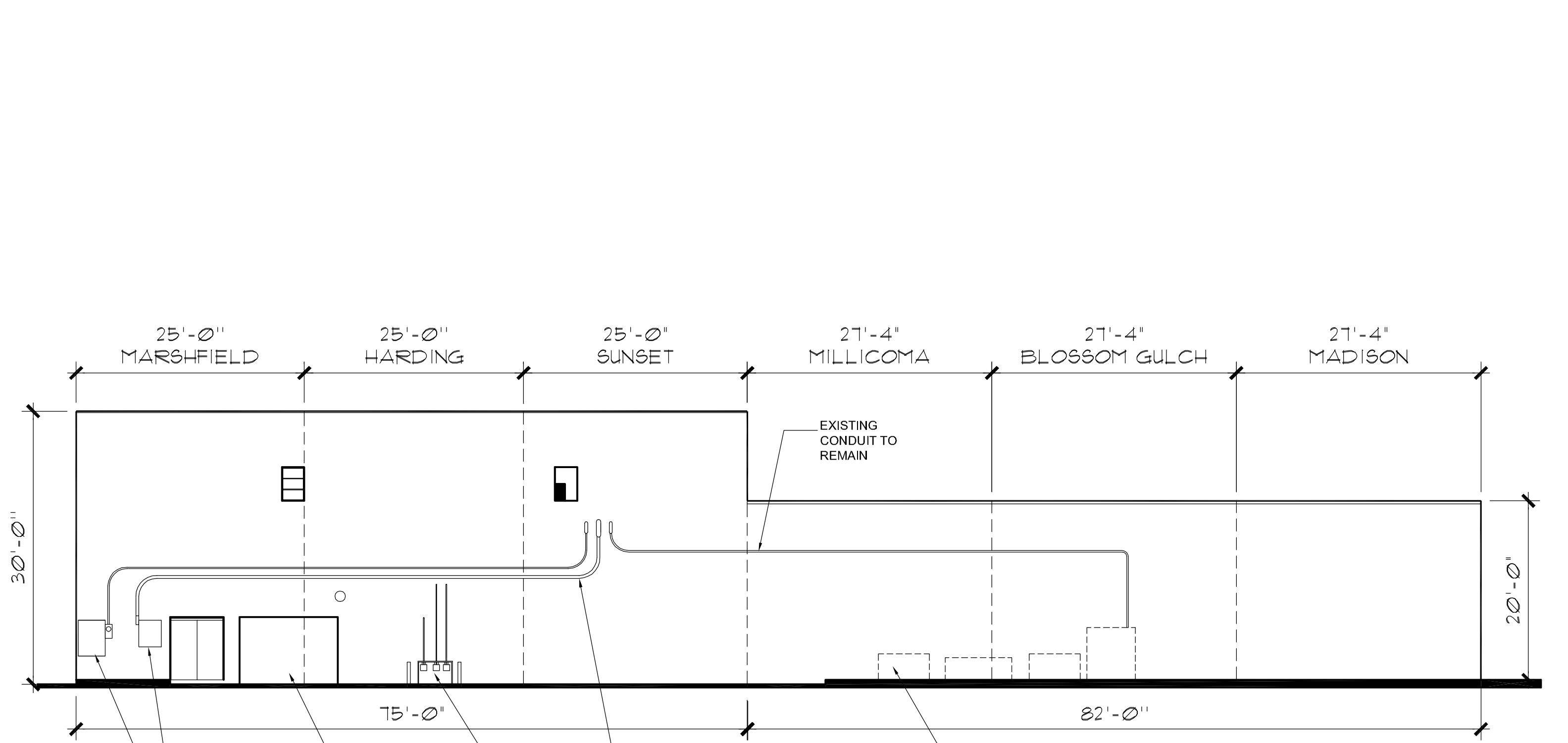
EAST ELEVATION NOTE: DIMENSIONS ARE APPROXIMATE 0 1 2 3 4 5 6 7 8 9 10 SCALE BAR
